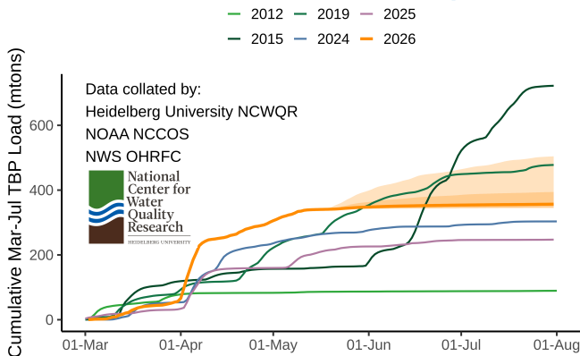
Fig. 2. Cumulative TBP loads for the Maumee River (Waterville, OH). Each line denotes cumulative load for different years. 2026 is in orange: the solid line is the measured load to May 11 and predicted load for the rest of the loading season (thru July); the darker and lighter orange shading show, respectively, the likely and possible load ranges for the remainder of the season.
