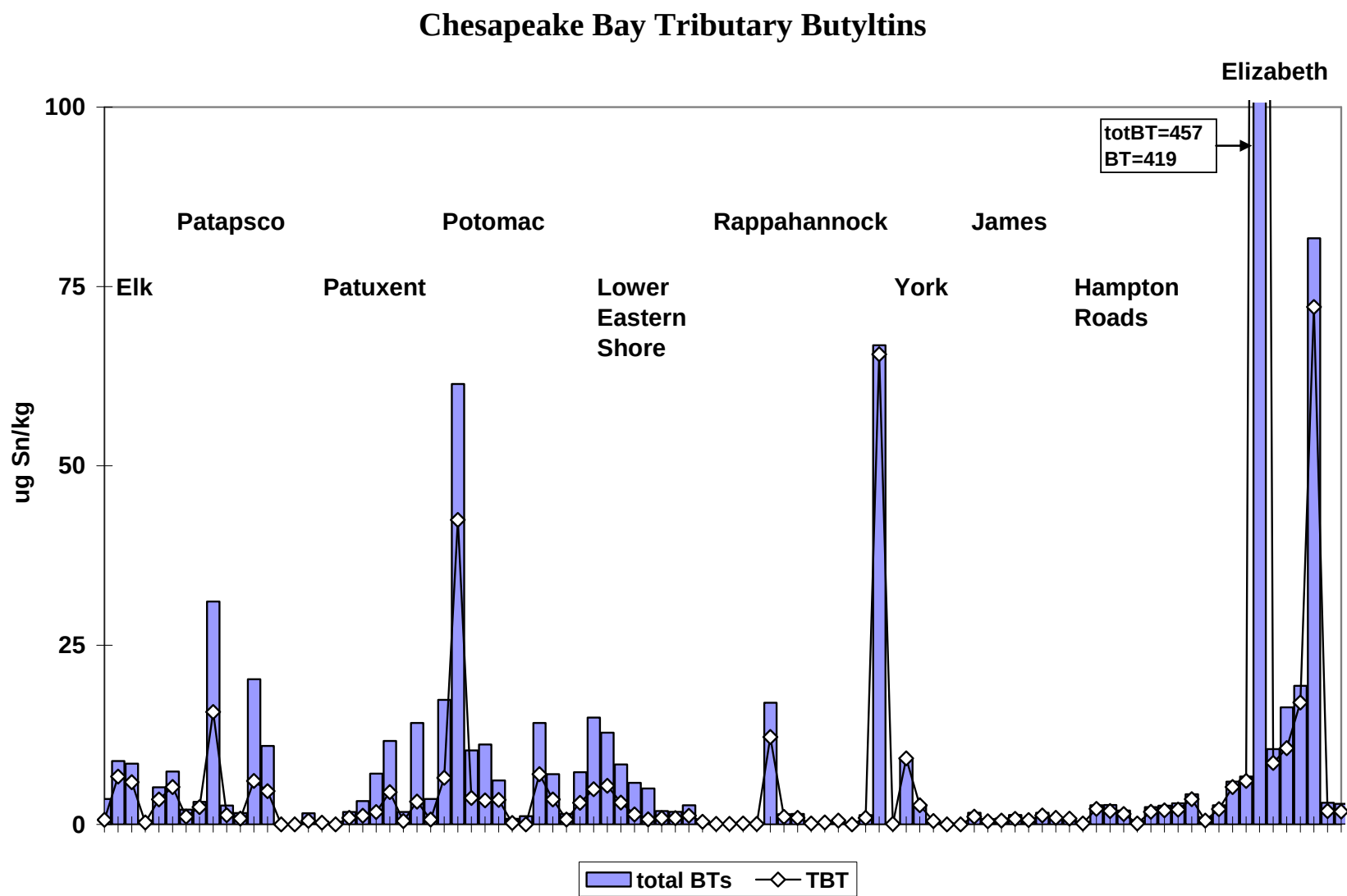
Figure 24c. Concentrations of total Butyltins (bars) and TBT (diamonds) in Chesapeake Bay tributaries. Selected locations are noted.
