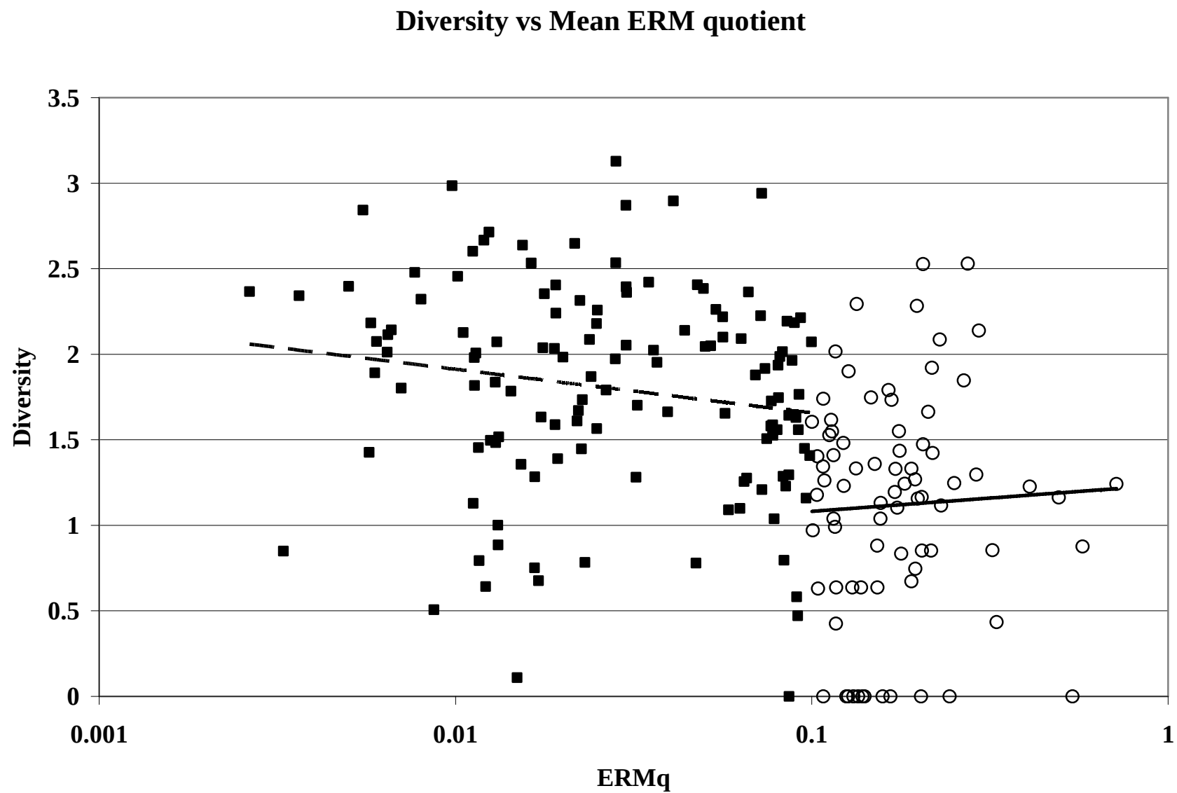
Figure 56. Relationship between species diversity and mean ERM quotient above and below a value of 0.1.
