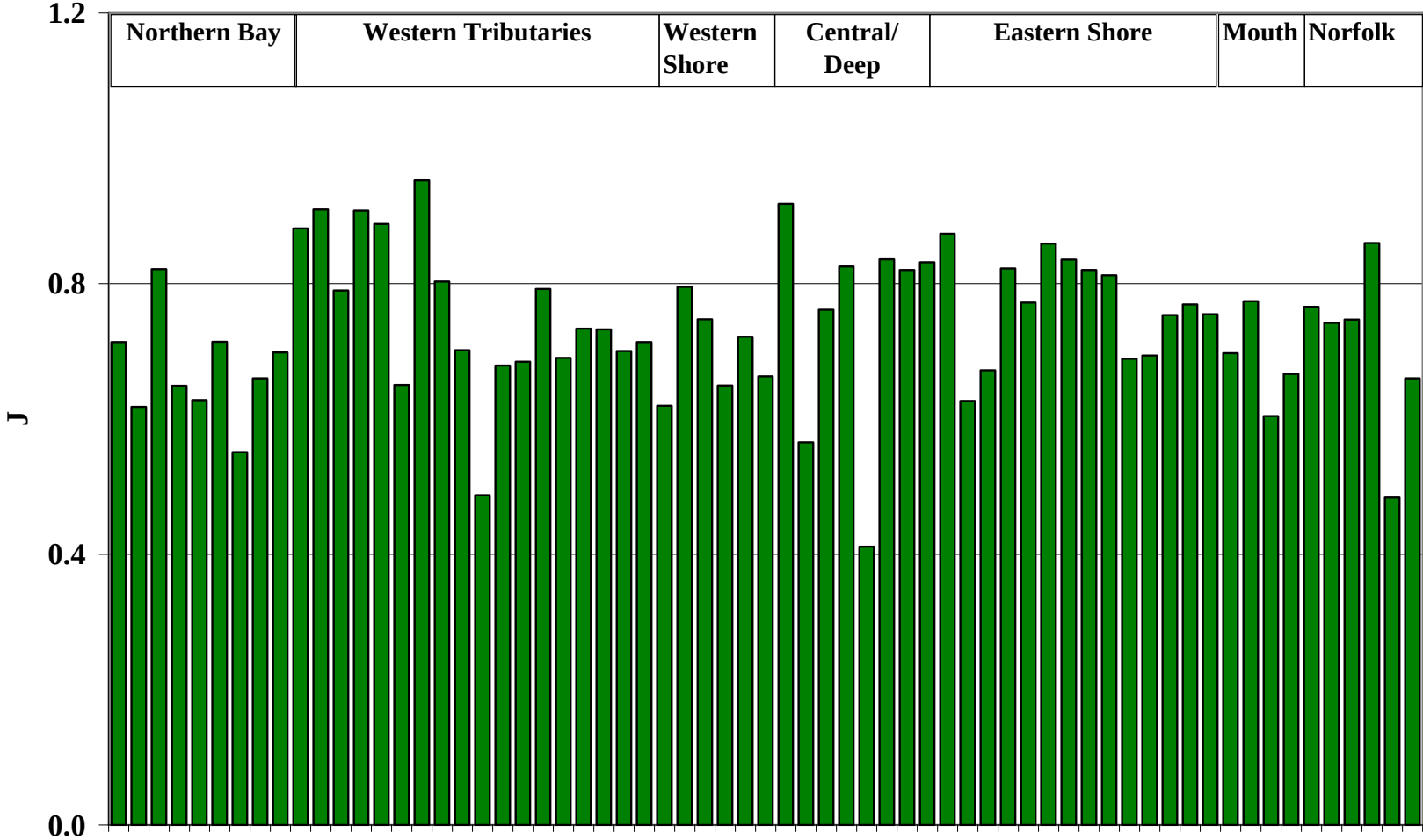
Figure 38. Species evenness in Chesapeake Bay sampling strata. Strata are arranged by region.
