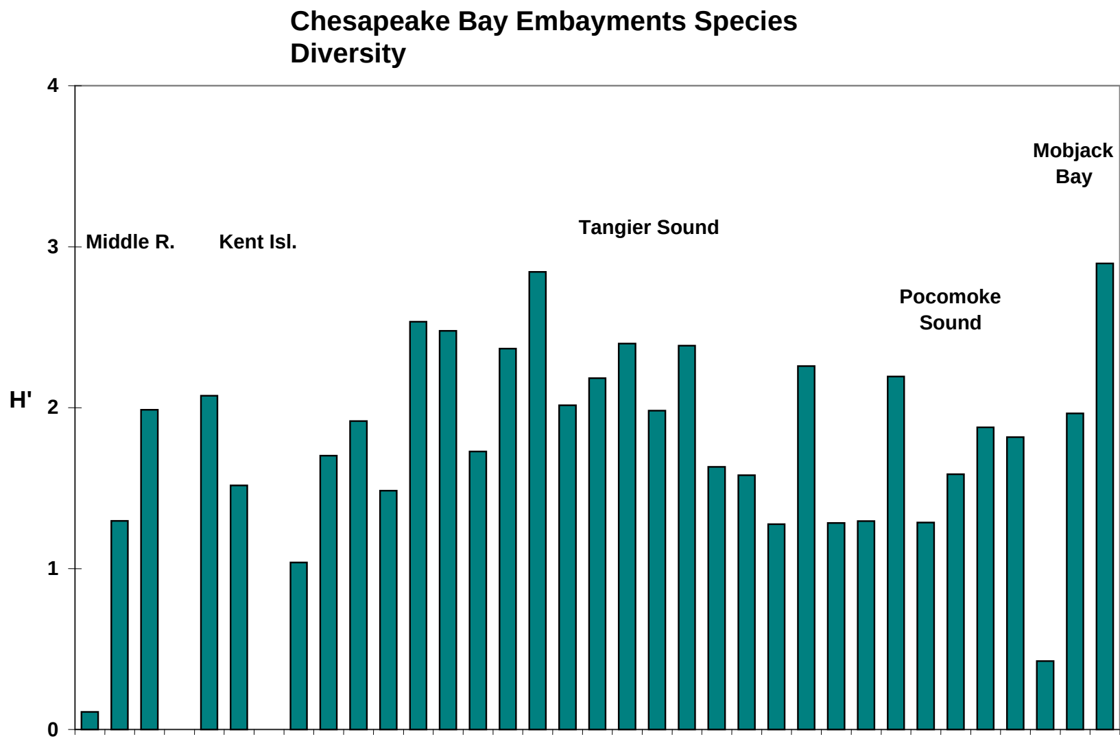
Figure 33b. Species diversity in Chesapeake Bay embayments. Selected locations are noted.
