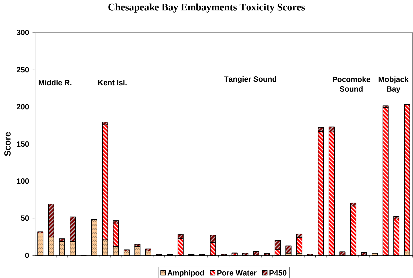
Figure 29b. Toxicity response scores from sediment bioassays of Chesapeake Bay embayments.
