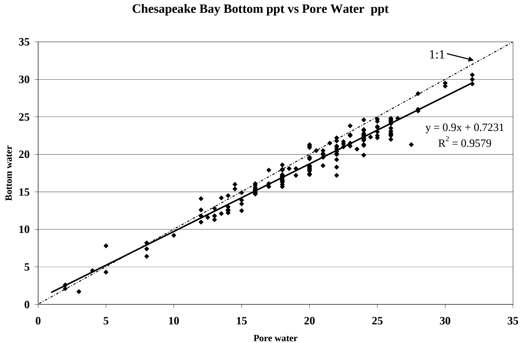
Figure 8. Correspondence of measured bottom water salinity and measured salinity of pore water (solid line).
