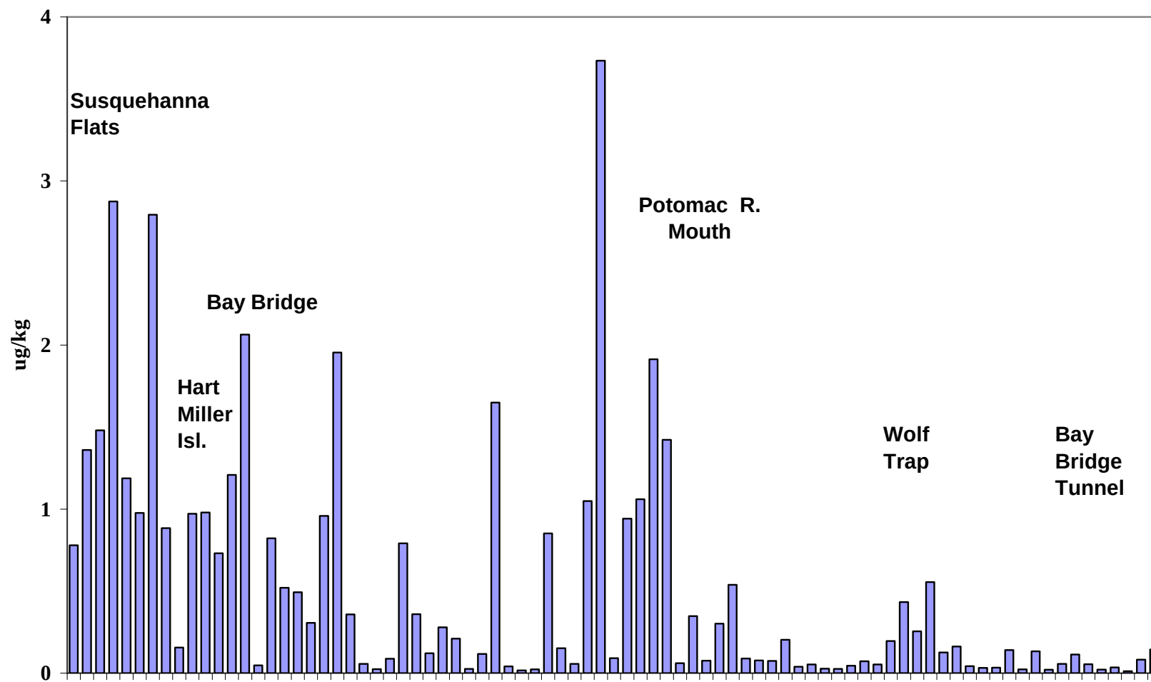
Figure 22a. Concentrations of chlorinated benzenes in the Chesapeake Bay mainstem. Selected locations are noted.
