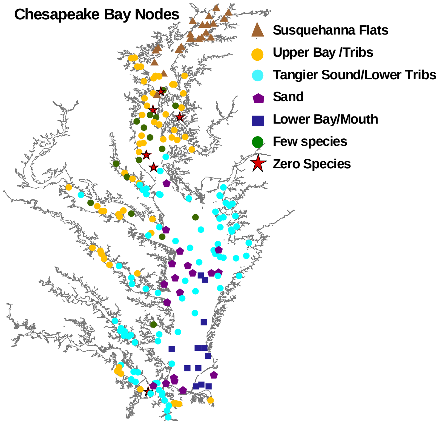
Figure 41. Distribution of species association nodes in Chesapeake Bay.
