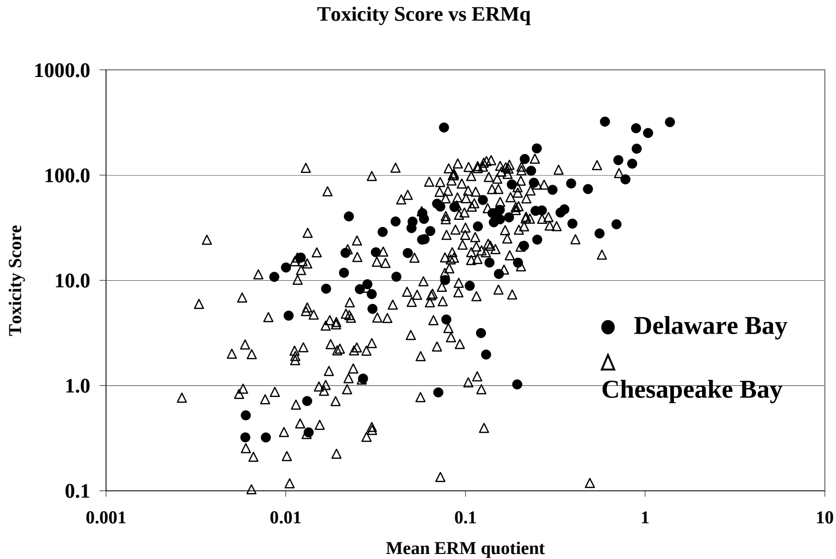
Figure 54. Relationship between observed toxicity response index and mean ERM quotient in independent studies of Delaware and Chesapeake Bays.
