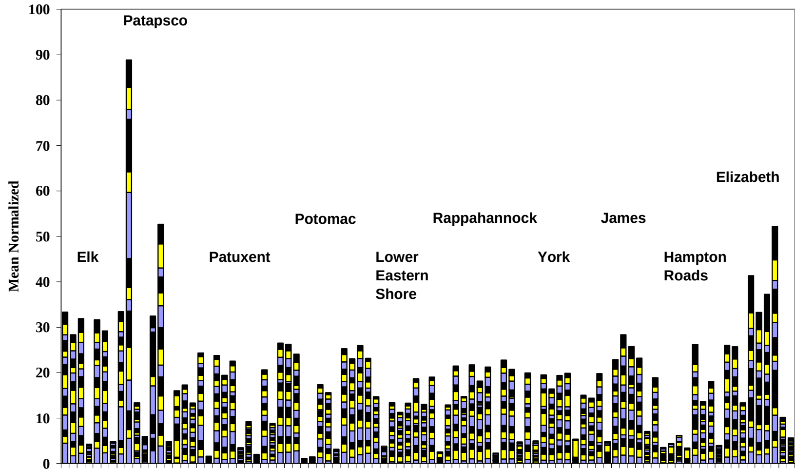
Figure 18c. Mean normalized concentrations of 15 elements (from bottom to top Ag, Al, As, Cd, Cr, Cu, Fe, Hg, Ni, Pb, Sb, Se, Sn, Tl, Zn) in Chesapeake Bay tributaries. Selected locations are noted.
