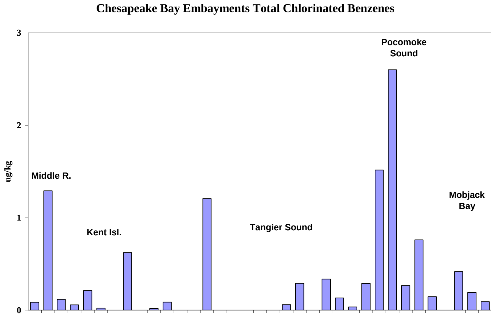
Figure 22b. Concentrations of chlorinated benzenes in Chesapeake Bay embayments. Selected locations are noted.
