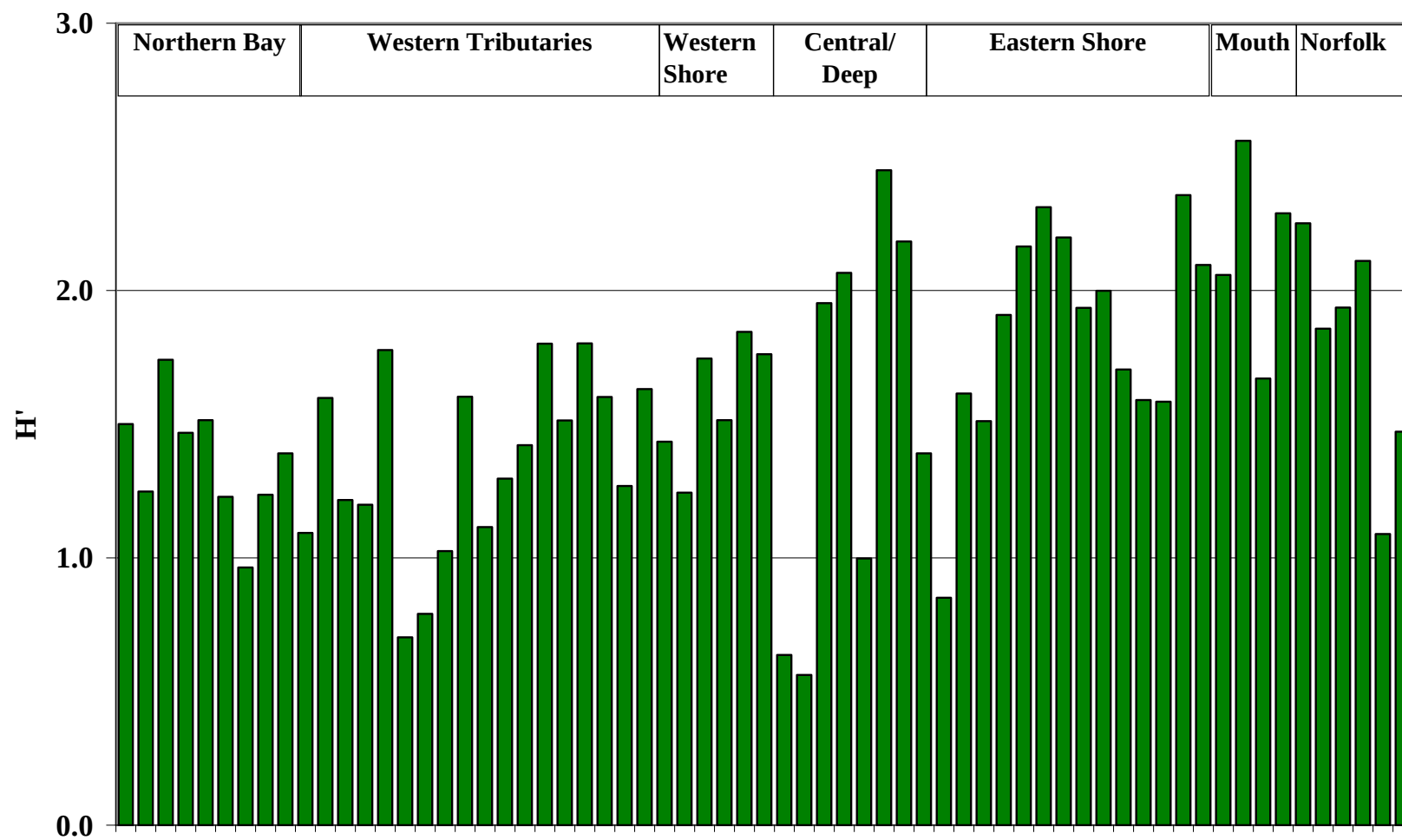
Figure 37. Species diversity in Chesapeake Bay sampling strata. Strata are arranged by region.
