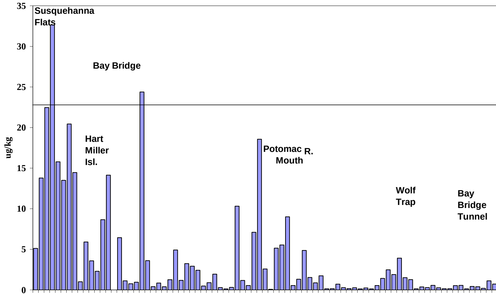
Figure 17a. Concentration of measured PCBs in the Chesapeake Bay mainstem. Selected locations are noted. Horizontal line indicates ERL concentration.
