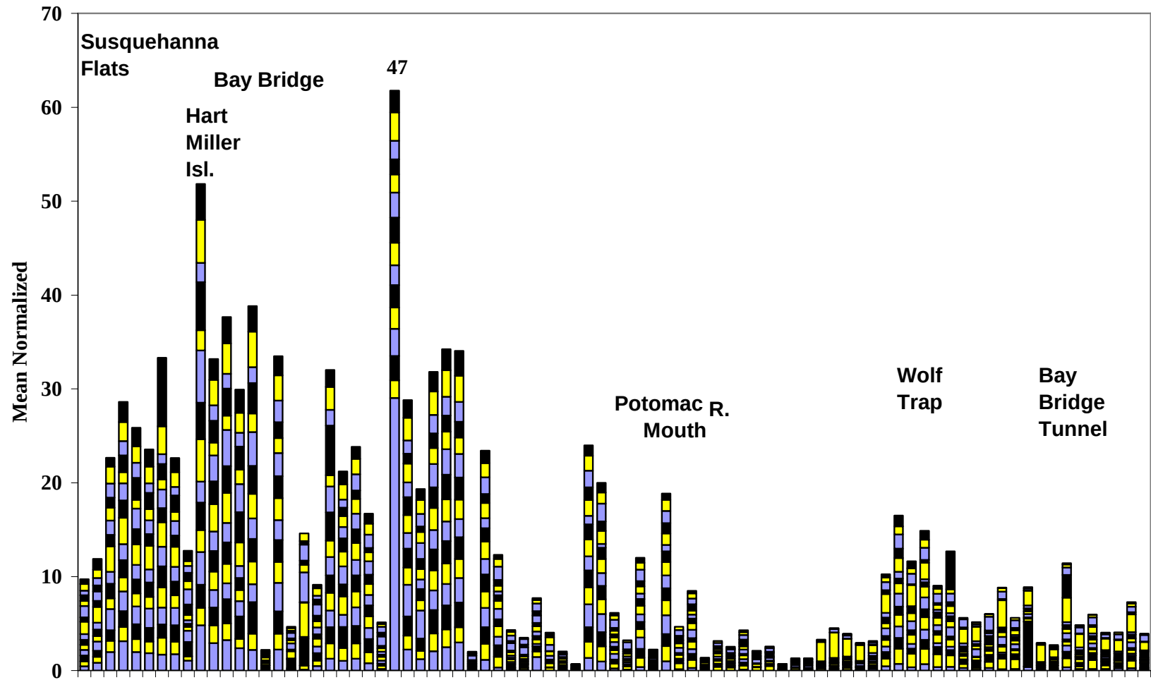
Figure 18a. Mean normalized concentrations of 15 elements (from bottom to top Ag, Al, As, Cd, Cr, Cu, Fe, Hg, Ni, Pb, Sb, Se, Sn, Tl, Zn) in the Chesapeake Bay mainstem. Selected locations are noted.
