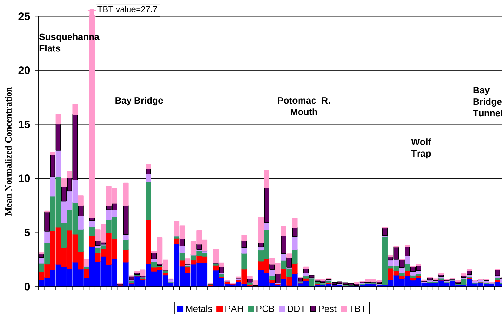
Figure 12a. Normalized sediment contaminant concentrations in the Chesapeake Bay mainstem. Selected locations are noted.
