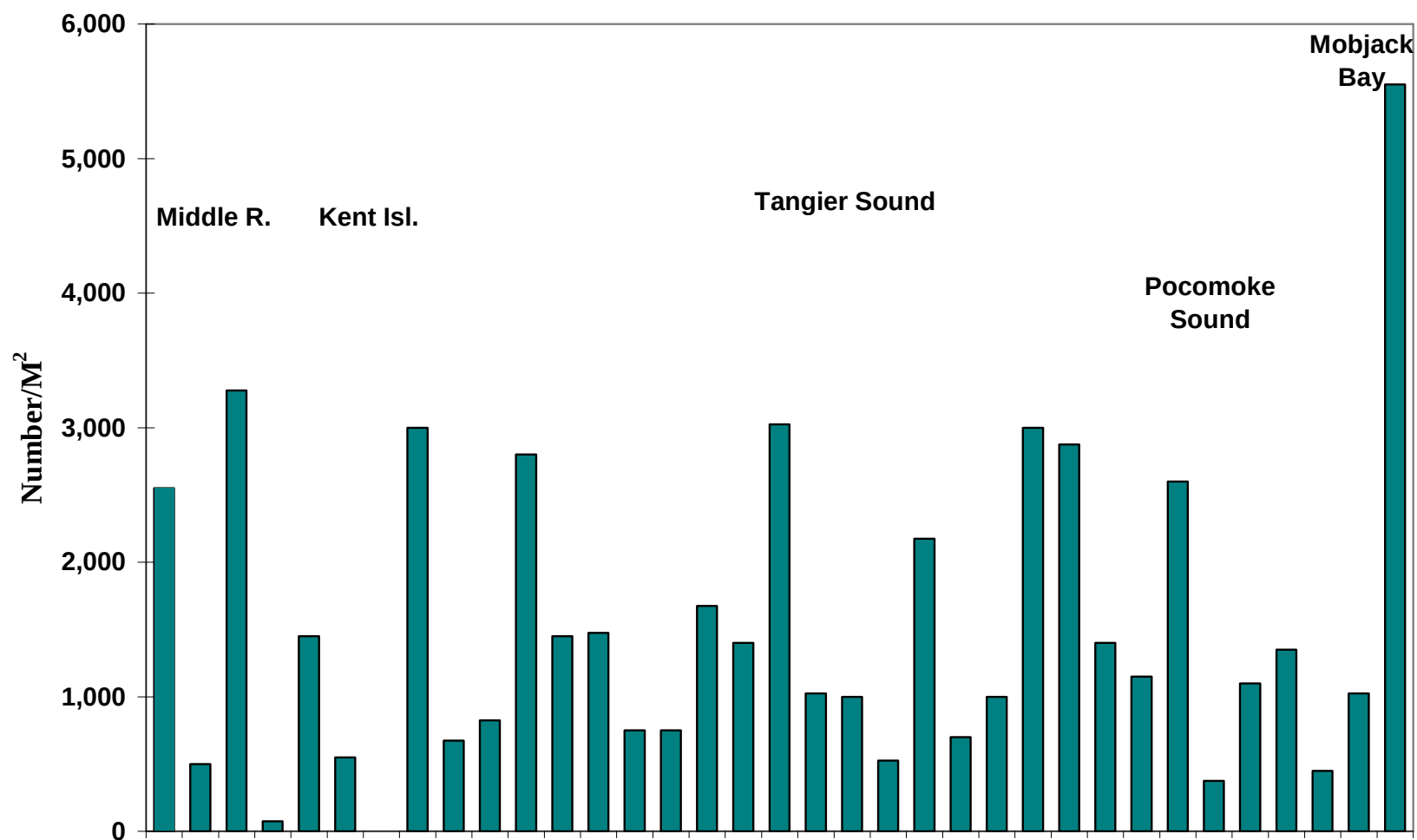
Figure 32b. Species abundance in Chesapeake Bay embayments. Selected locations are noted.
