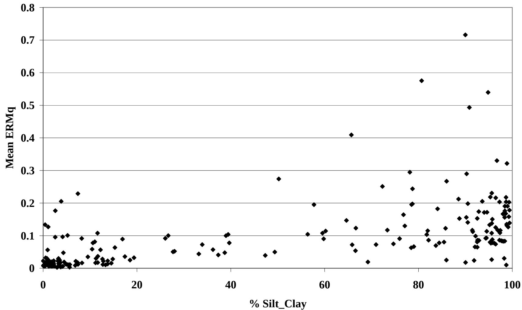
Figure 57. Relationship between mean ERM quotient and grain size in Chesapeake Bay sediments.
