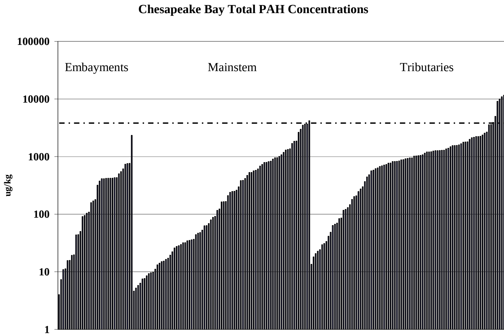
Figure 13. Total PAH concentrations in Chesapeake Bay sediment samples. Dashed line indicates ERL concentration.
