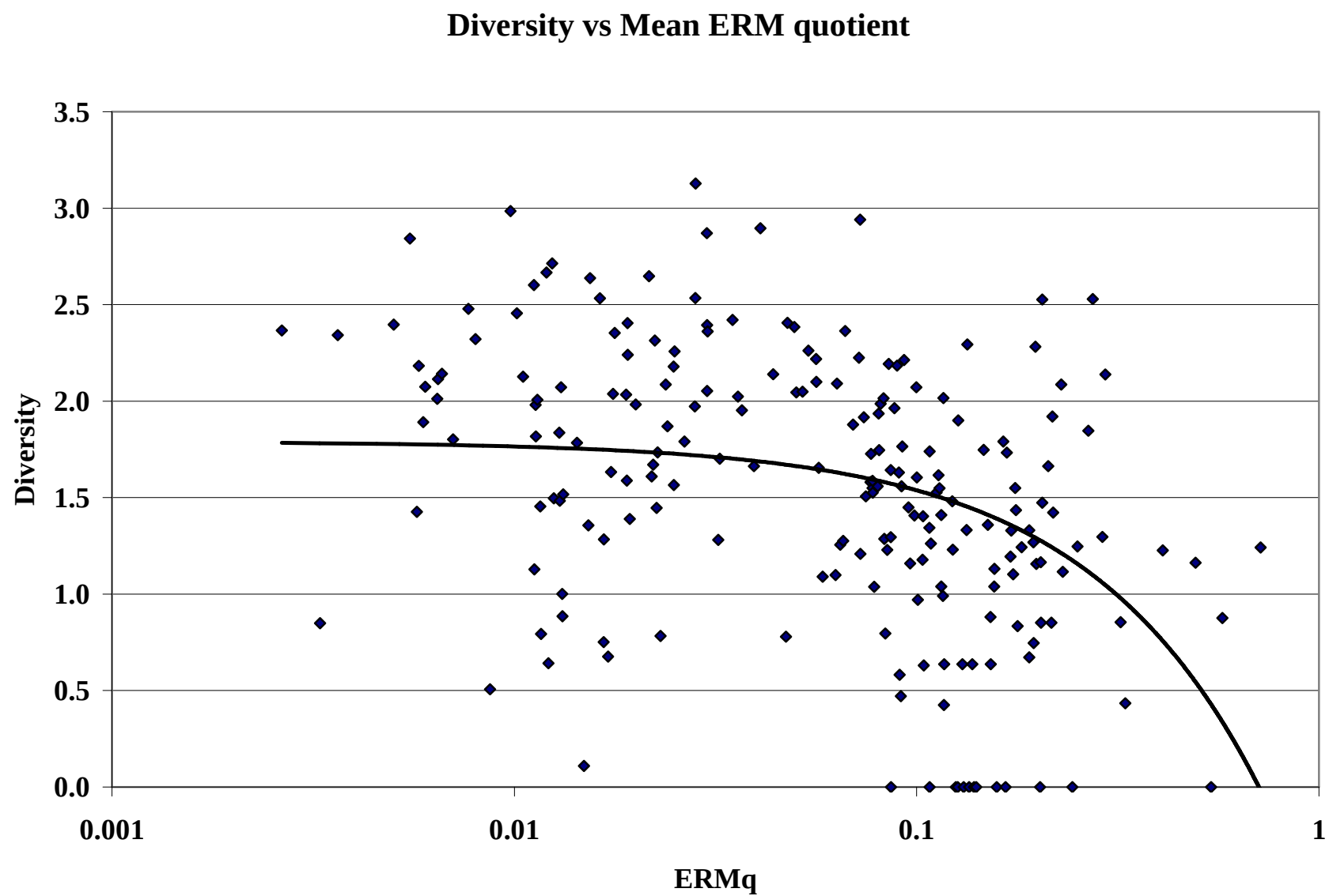
Figure 55. Relationship between species diversity and mean ERM quotient values in sediment samples from Chesapeake Bay.
