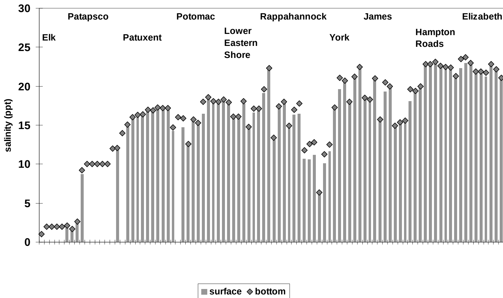
Figure 9c. Surface and bottom salinity in Chesapeake Bay tributaries. Selected locations are noted.
