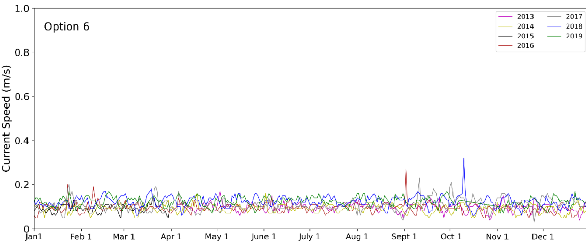
Figure 45. Northeast Planning Area, option 6 Navy Coastal Ocean modeled oceanographic features from 2013 to 2019 at the surface for water temperature (top panel), salinity (middle panel), and current speed (bottom panel).
