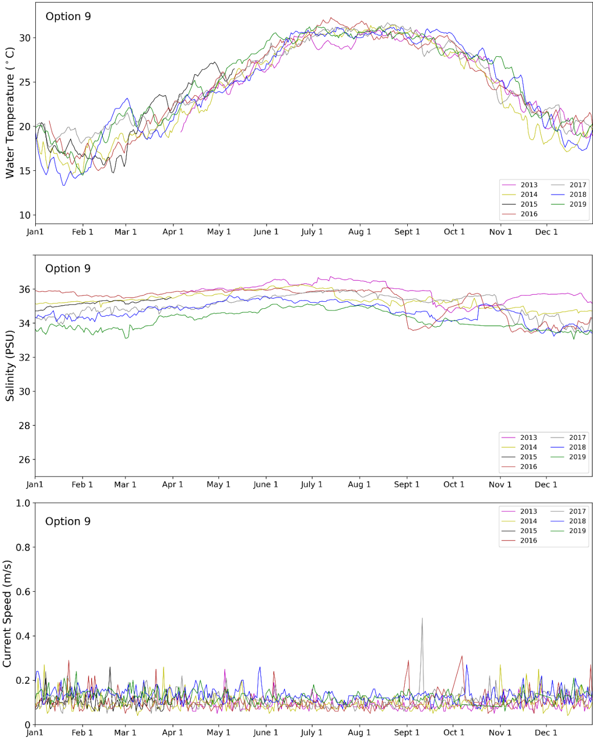
Figure 54. South A Planning Area, option 9 Navy Coastal Ocean modeled oceanographic features from 2013 to 2019 at the surface for water temperature (top panel), salinity (middle panel), and current speed (bottom panel).
