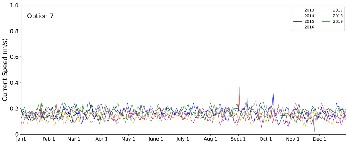
Figure 47. Northeast Planning Area, option 7 Navy Coastal Ocean modeled oceanographic features from 2013 to 2019 at the surface for water temperature (top panel), salinity (middle panel), and current speed (bottom panel).
